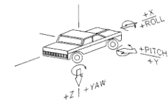
Figure C2. Vehicle Angular Displacements for Test No. 467824-1.
